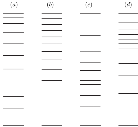
Figure 1. Energy levels of the n single phonon states |0, \dots, 0, 1, 0, \dots, 0\rangle , for n = 12 . In each of the cases, \hbar = \omega = 1 . The four cases correspond to: (a) a Hamiltonian (4) with constant nearest-neighbour interaction (for c = 0.5 ); (b) a Hamiltonian with Krawtchouk interaction (39) or with Hahn interaction (52) (for c = 0.18 ); (c) a Hamiltonian with q -Krawtchouk interaction (65) where q > 1 (here, q = 1.6 and c = 1.0 ); (d) the same q -Krawtchouk interaction (65) where 0 < q < 1 (here, q = 0.7 and c = 0.01 ). The levels are rescaled, so that the lowest and highest levels match in the four cases.
